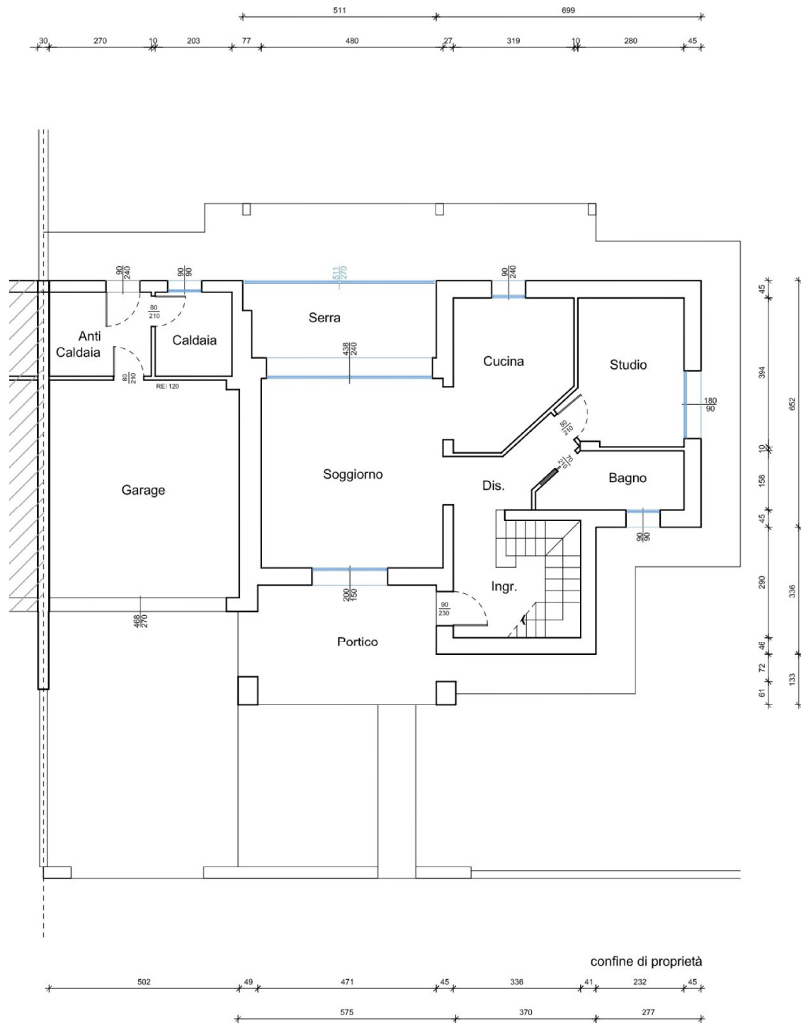
PIANO TERRA
